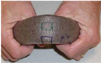
Figure 12: Foam Rod Failure
