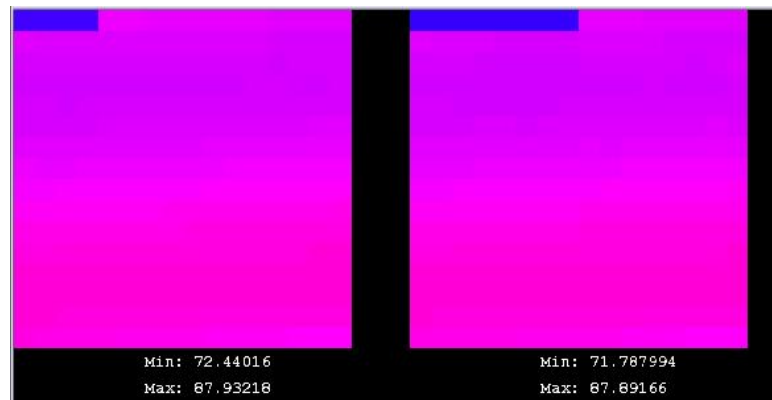
Figure 3. Difference in S-arrays with the first bytes of the key the same.
