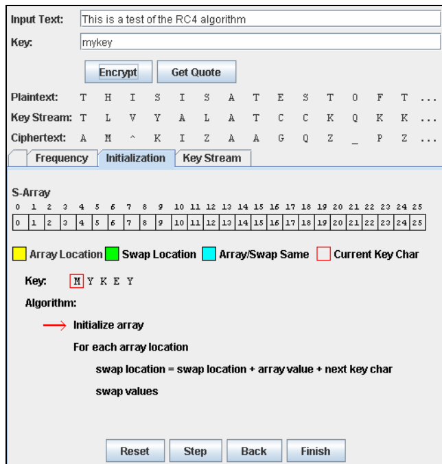
Figure 2. RC4 visualization applet.
